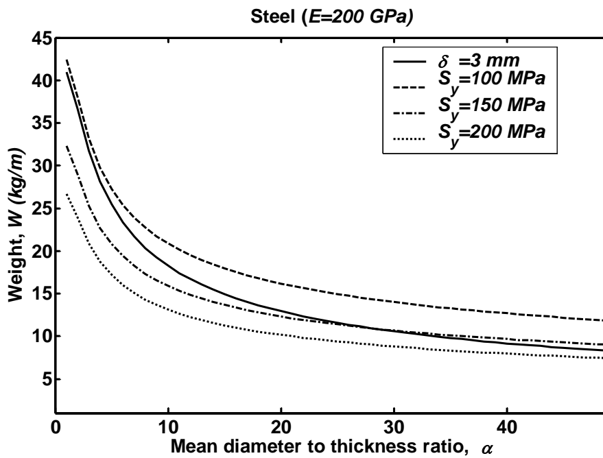
Fig.4 Variation of beam weight, W , vs. mean diameter-to-thickness ratio, \alpha
