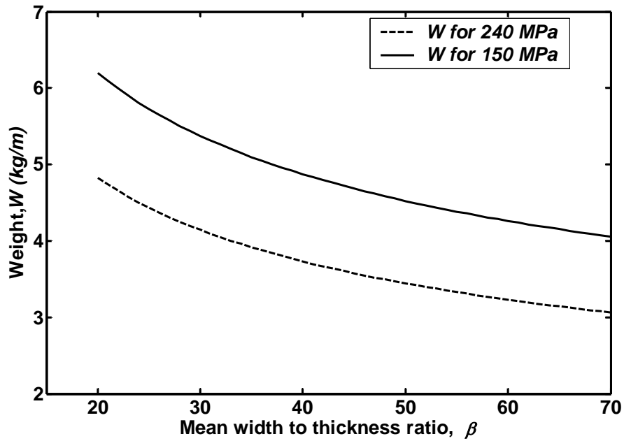
Fig. 8 Weight, W vs. mean width to thickness ratio, \beta
