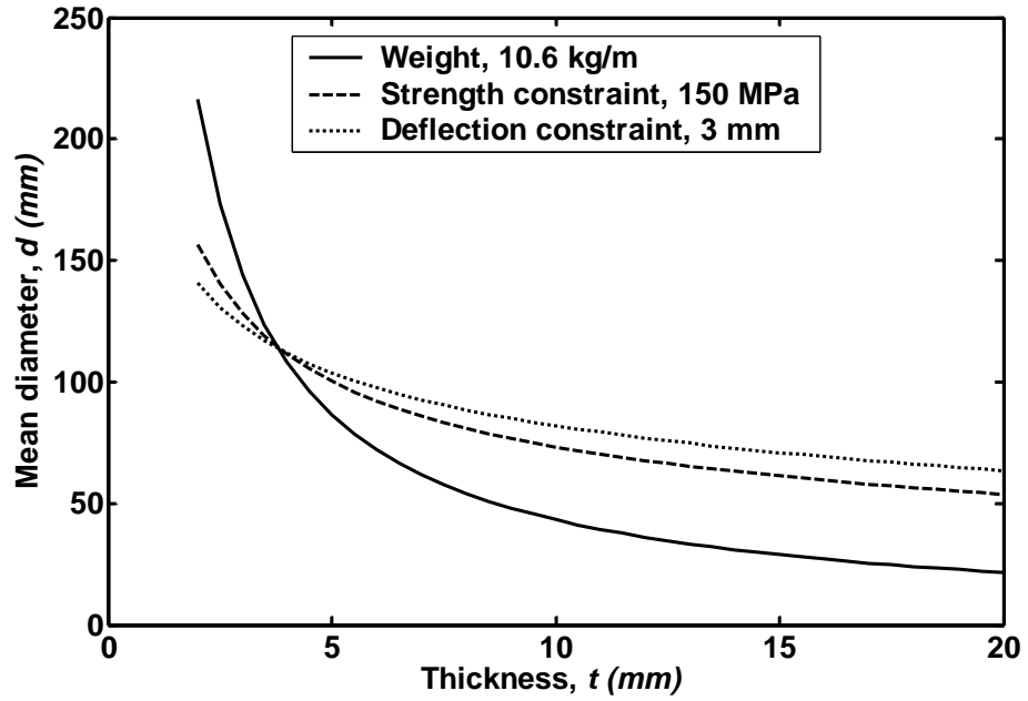
Fig. 5 Contour of objective function and the constraints in design variable space
