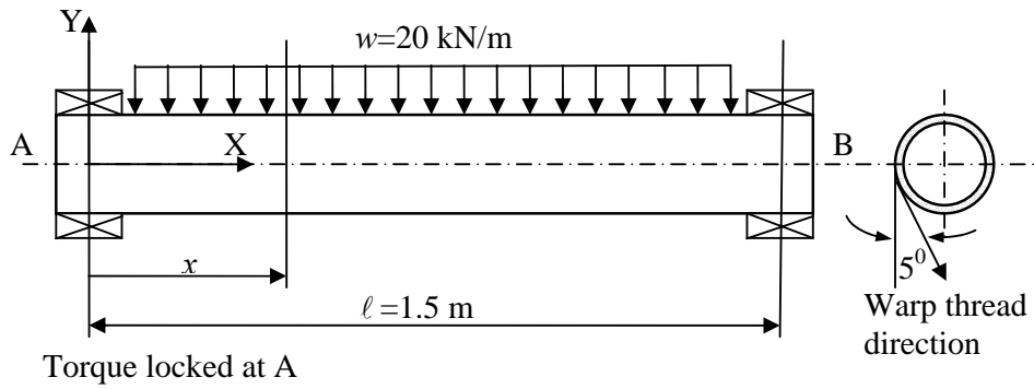
Fig. 3 Load diagram of the upper (warp) beam
