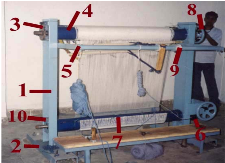
1. Support Channel; 2. Base Channel; 3. Ratchet; 4. Upper (Warp) Beam; 5. Shedding Pipe; 6. Tensioning Device; 7. Lower (Cloth) Beam; 8. Handle; 9. Shedding Roller; 10. Bush Bearing.
