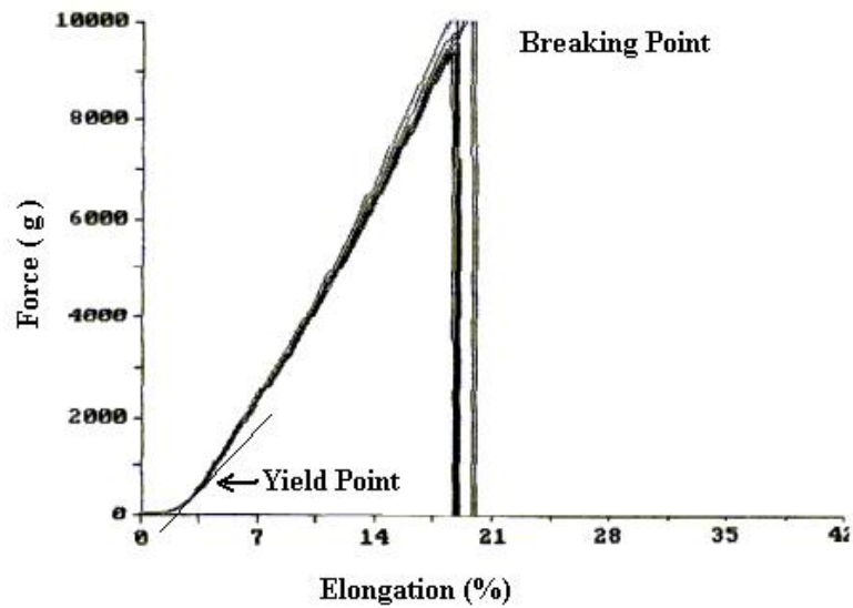
Fig. 2 Tensile test results of warp threads
